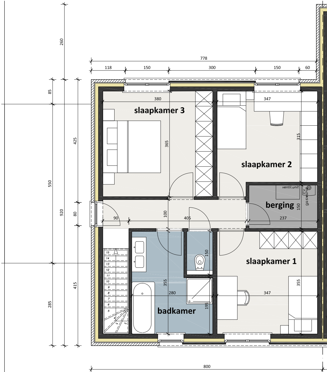
VERDIEPINGSPLAN - LOT 9
